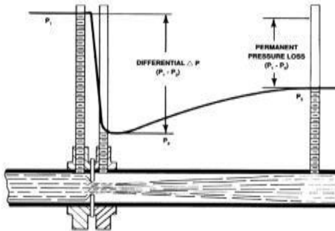
Typical Orifice Flow Pattern Flange Taps Shown
